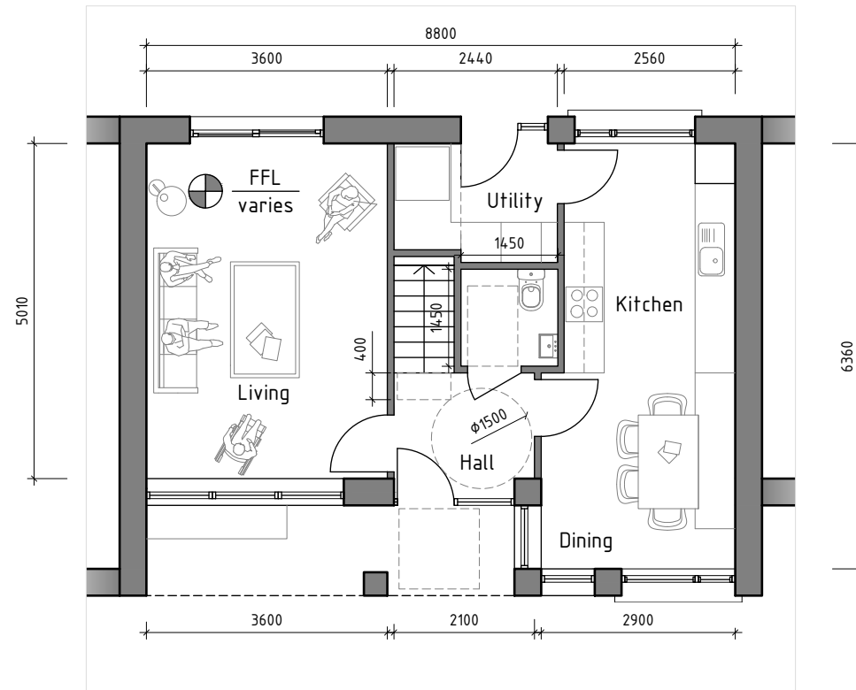
1 2-BED GROUND FLOOR PLAN PROPOSED 1:100@A3
